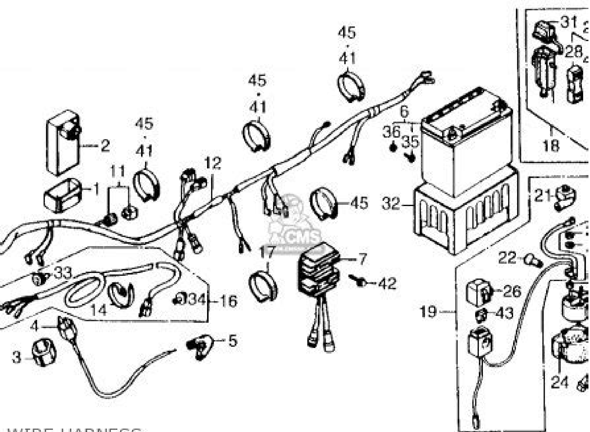
WIRE HARNESS
