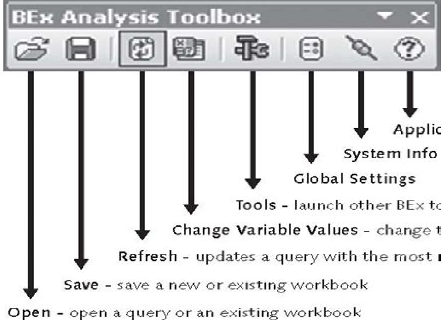
Figure 1.11 BEx Analyzer—Analysis Toolbar
