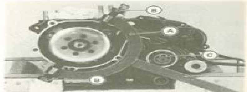
A. Rotor Holder: 57001-308 C. Sleeve B. Adapter "A": 57001-1108
