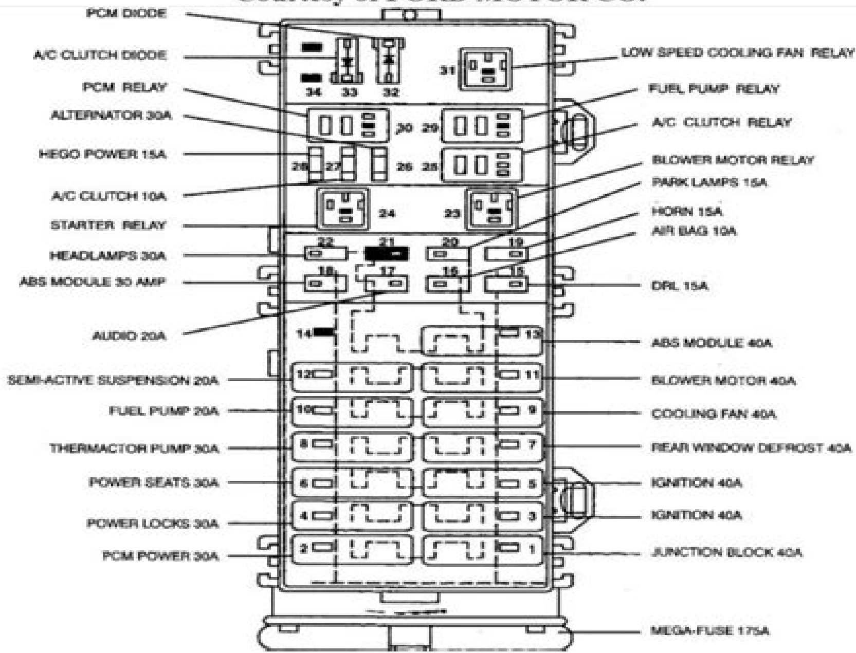
Fig. 6: Identifying Battery Junction Box Components Courtesy of FORD MOTOR CO.
