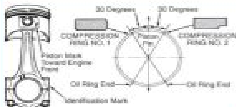
Fig. 17. Assembling Rings, Rod & Piston Courtesy of KIA MOTORS AMERICA, INC.
