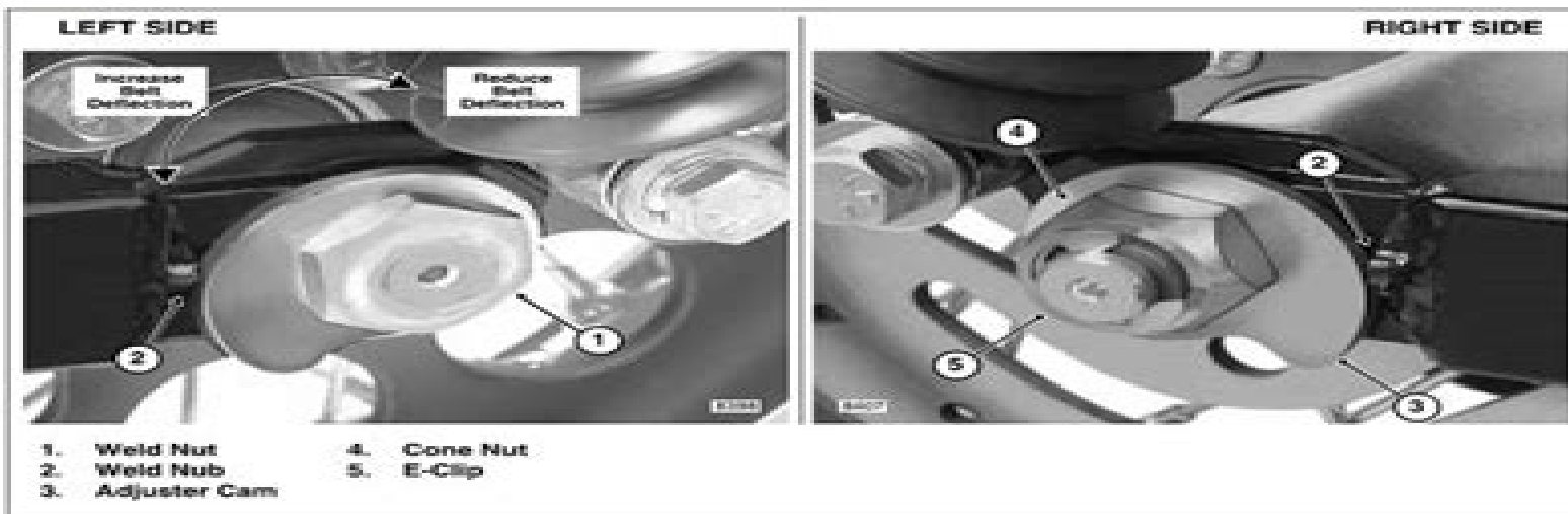
Figure 2-17. Move Rear Wheel Forward Until Adjuster Cams Just Contact Weld Nubs
