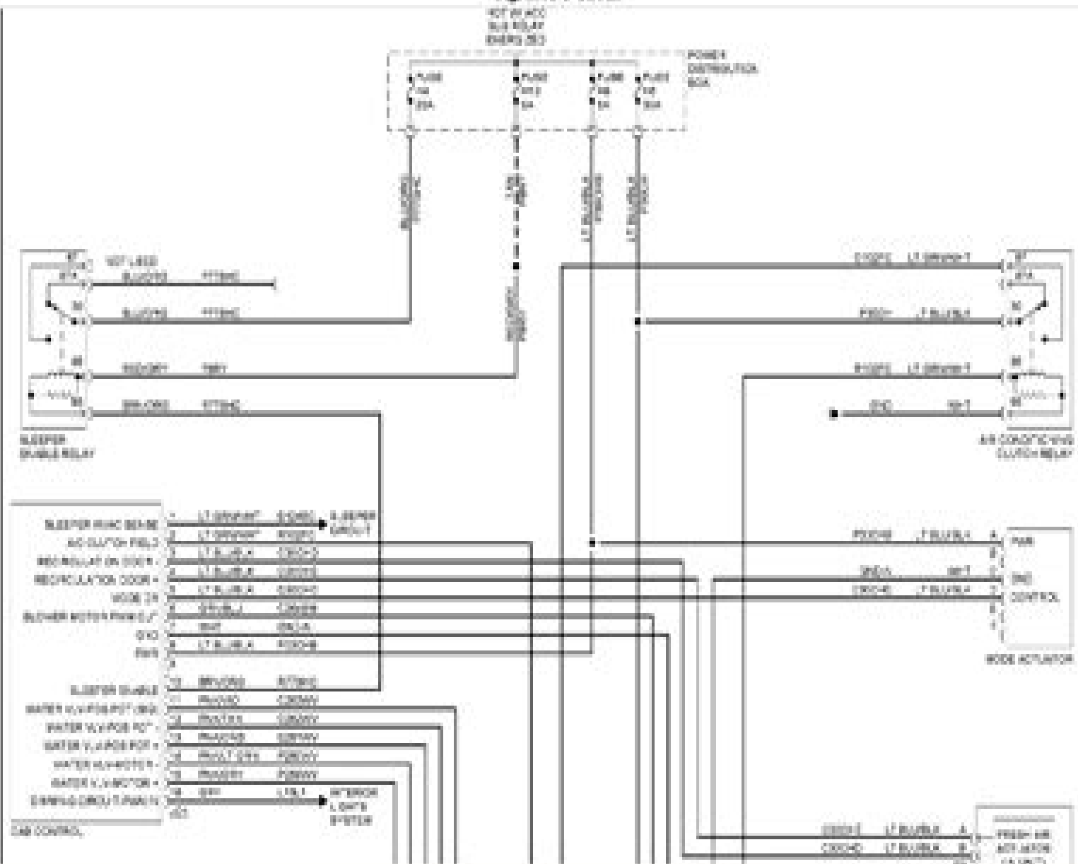
Fig. 1: AC Circuit
