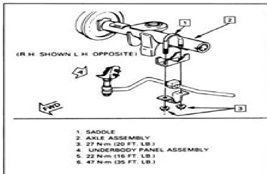
Figure 10 - Stabilizer Shaft
