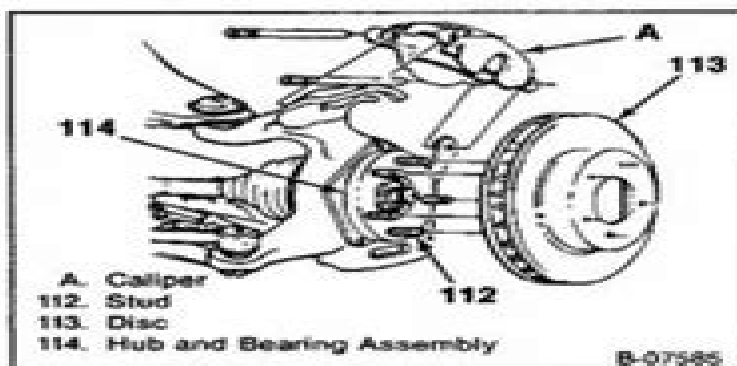
Figure 39—Removing the Disc
