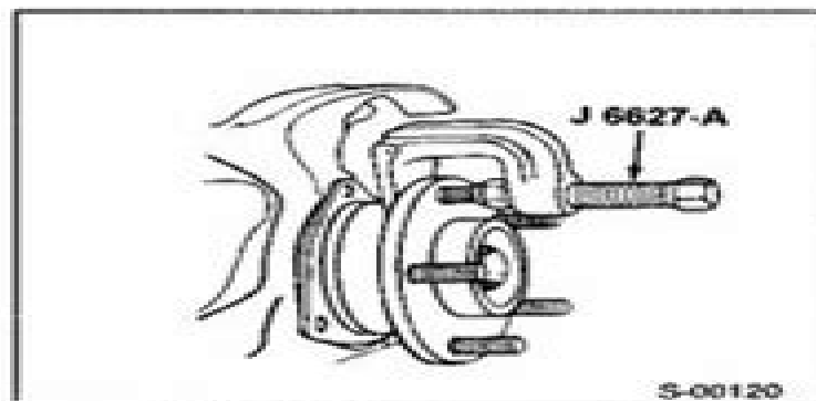
Figure 40—Removing the Wheel Studs
