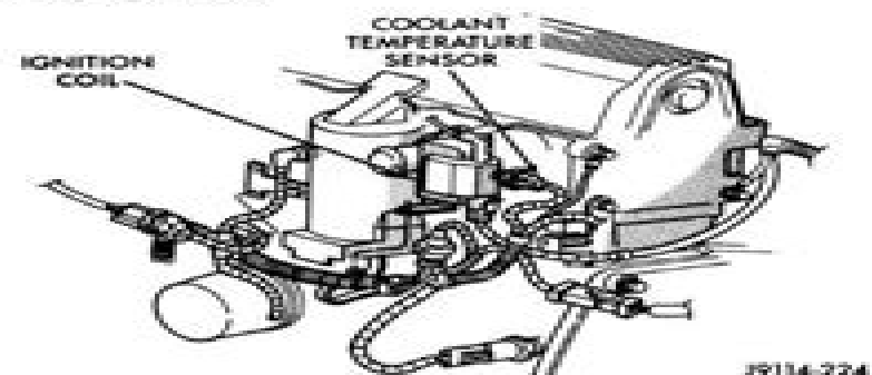
Fig. 23 Ignition Coil—2.5L Engine
