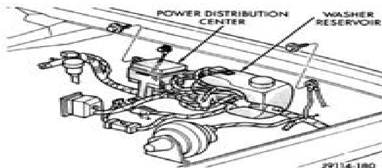
Fig. 22 ASD Relay
