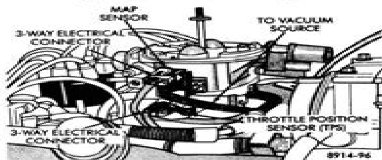
Fig. 21 MAP Sensor—3.9L and 5.2L Engines
