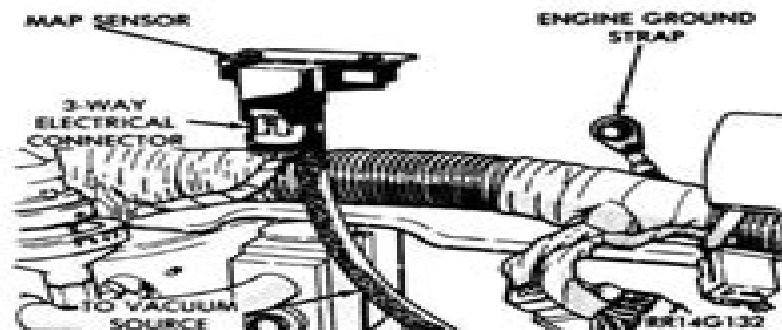
Fig. 20 MAP Sensor—2.5L Engine
