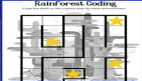
RainForest Coding
