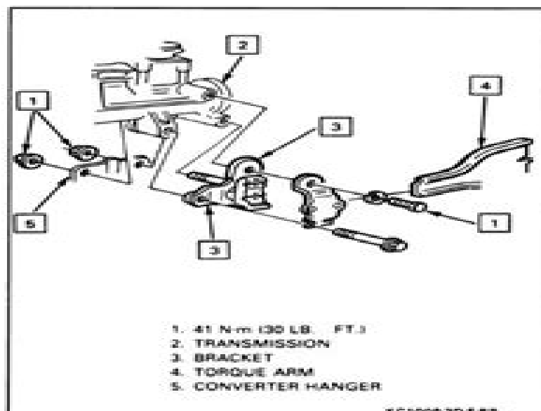
Figure 9 - Torque Arm Attachment-Manual Transmission
