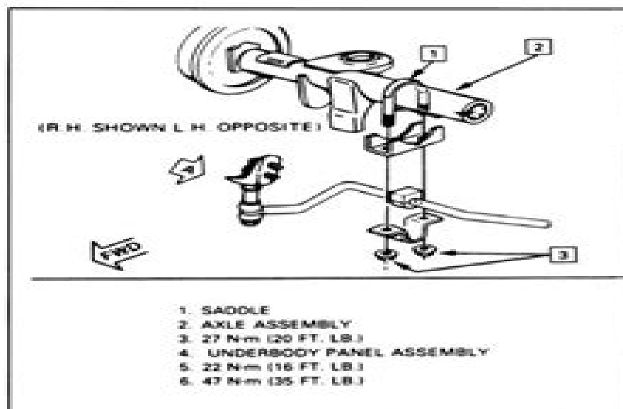
Figure 10 - Stabilizer Shaft
