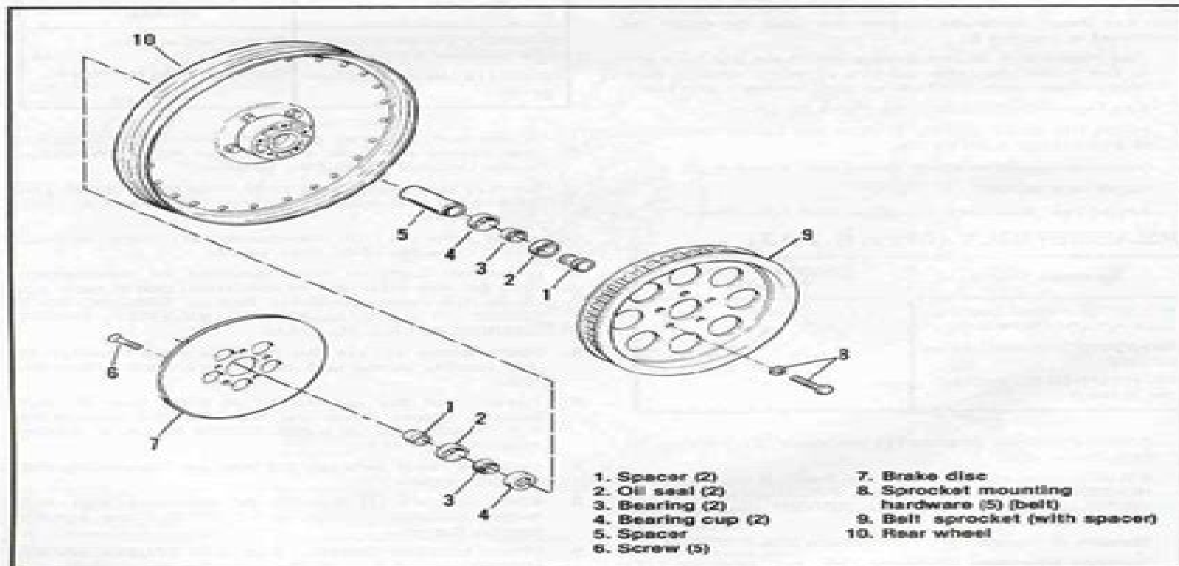
Figure 2-15. Rear Wheel - Disc
