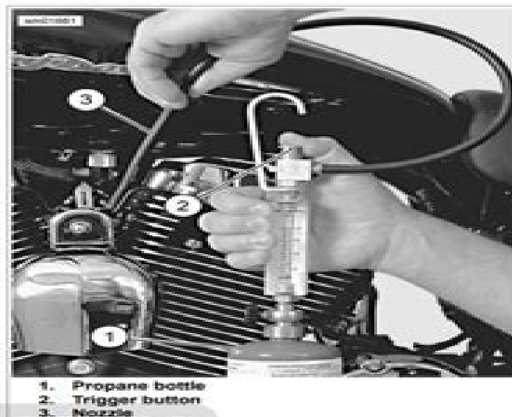
Figure 4-85. Checking for Leaks: All Models
