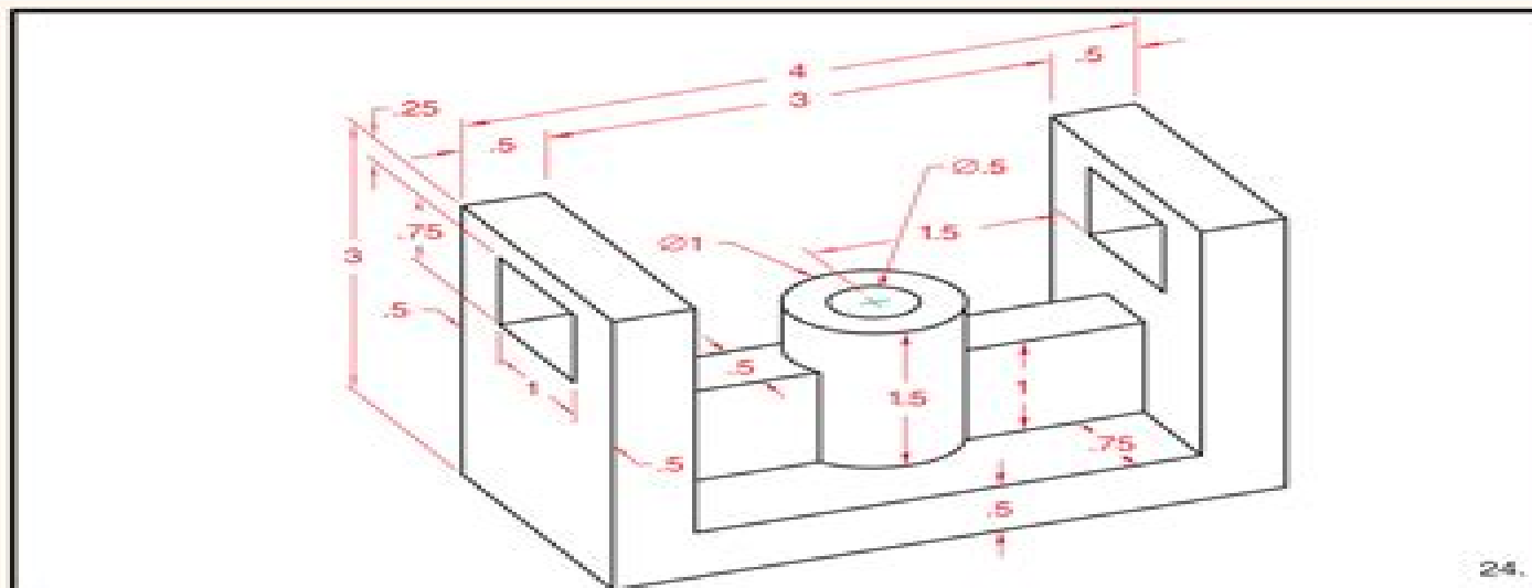
Problem 10-24. *** Bearing Cradle. Draw the necessary views and correctly dimension them.
