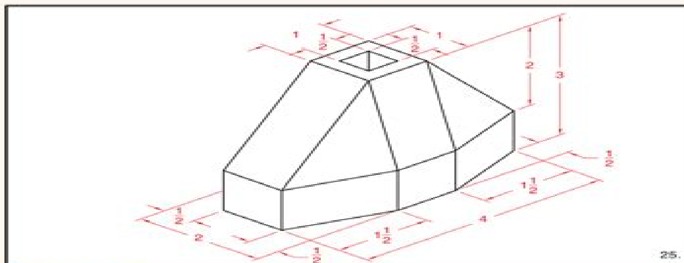
Problem 10-25. *** Pedestal Base. Draw the necessary views and correctly dimension them.
