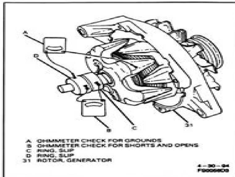
Figure 5 - Testing Generator Rotor
