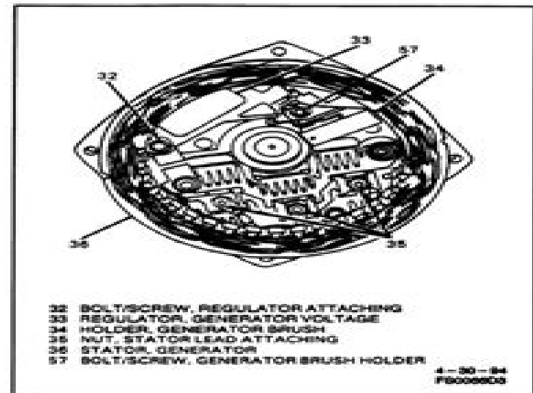
Figure 6 - Generator Slip Ring End Frame View
