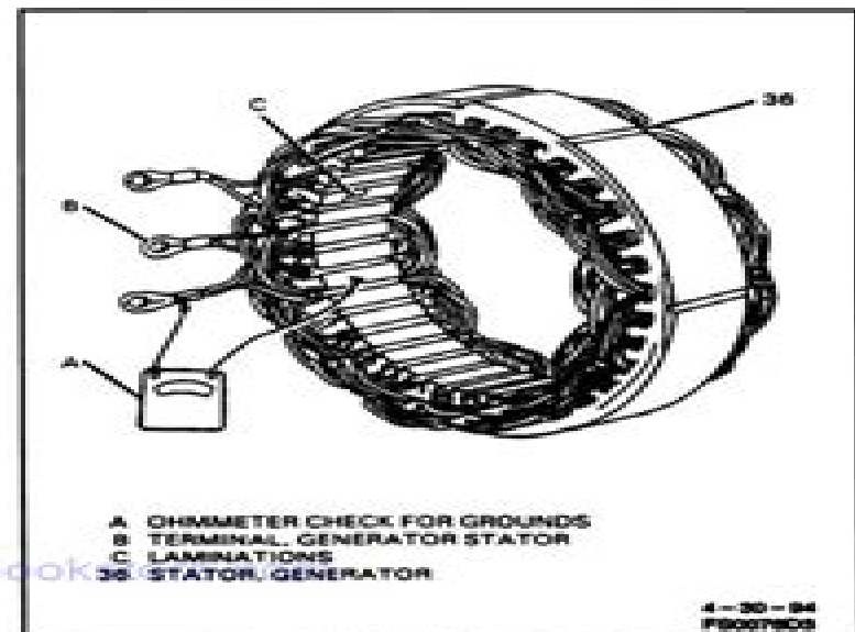
Figure 7 - Testing Generator Stator
