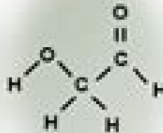
Glycolaldehyde
