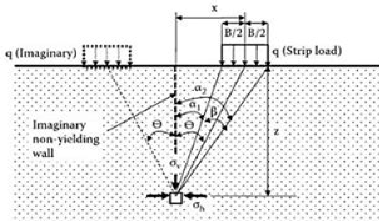
FIGURE 12.30 Boussinesq's lateral stress against nonyielding wall due to strip load.
