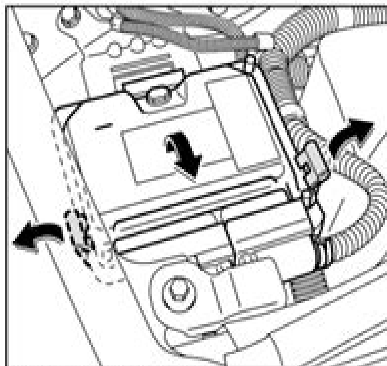
Fig. 5: Removing DME control module
