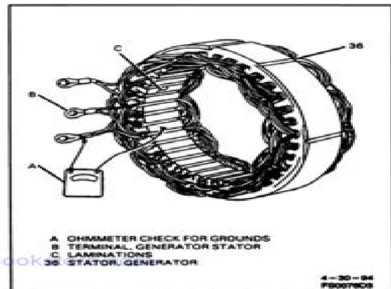
Figure 7 - Testing Generator Stator
