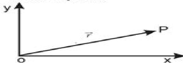
Fig 2.3: Position vector.
