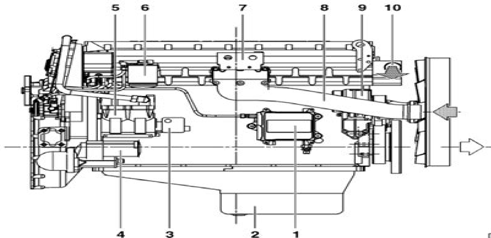
RIGHT SIDE
