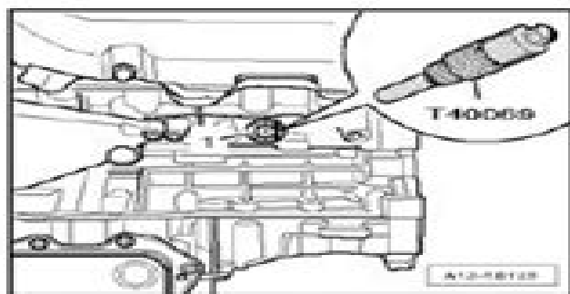
Fig. 335: Inserting Crankshaft Pin T40069 Into Hole
