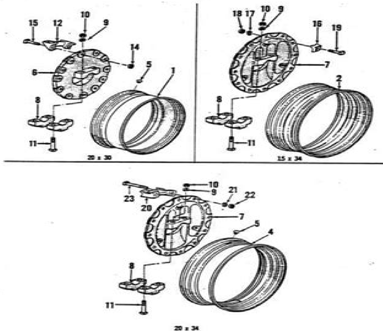
FIG. 181 - STANDARD REAR WHEELS 9000 (7448-75)
