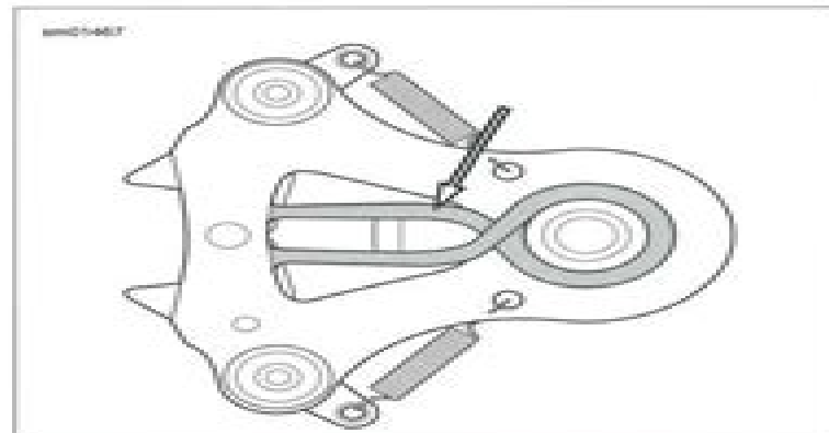
Figure 5-72. Correctly Installed Shifter Shaft Return Spring
