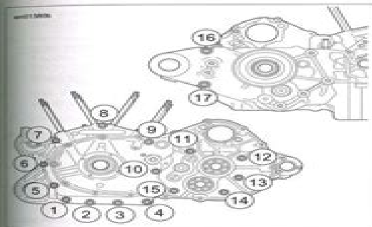
Figure 5-71. Crankcase Fastener Torque Sequence
