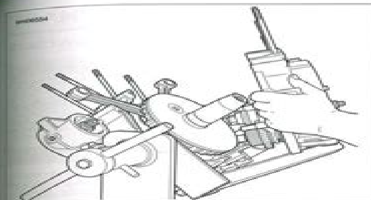
Figure 5-70. Assembling Crankcases With Crankshaft Guide Tool (Part No. HD-42325-A)
