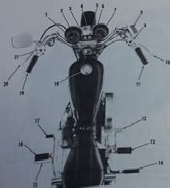
FIGURE 5. TOP VIEW, MODEL XLCH-1000
