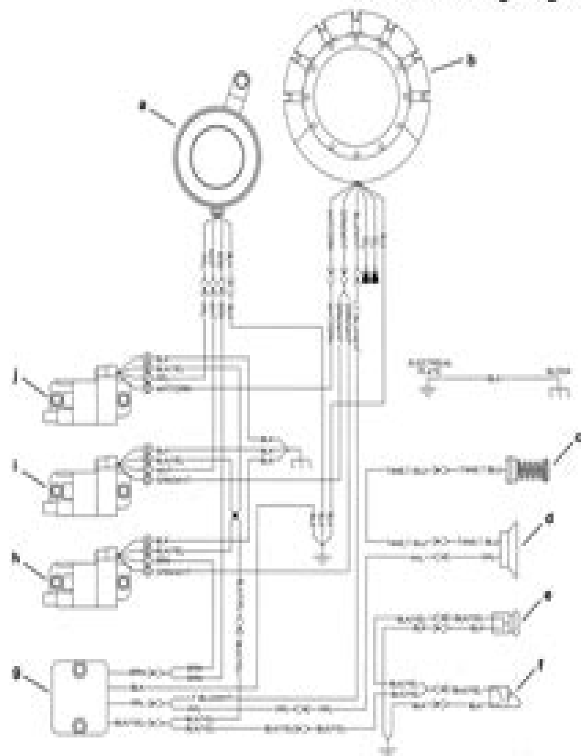
40/55 MM Wiring Diagram
