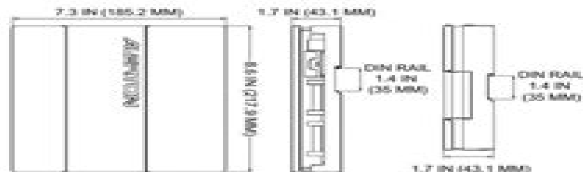
Fig. 1 ACM mounting dimensions.
