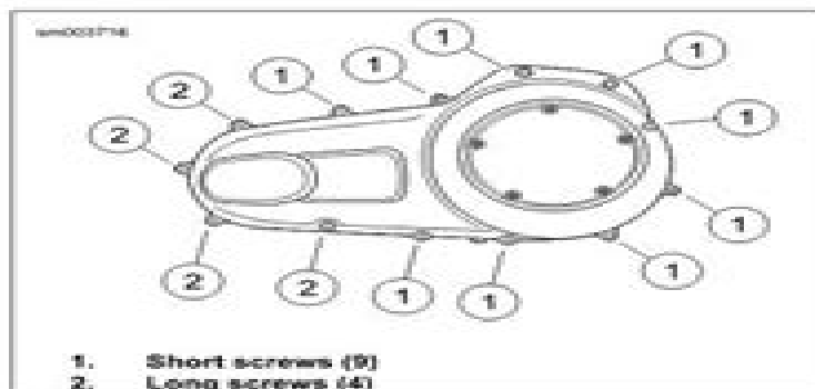
Figure 7-1. Primary Chaincase Cover Screws
