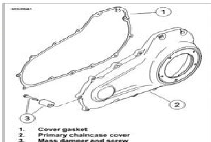
Figure 7-2. Primary Chaincase Cover Gasket
