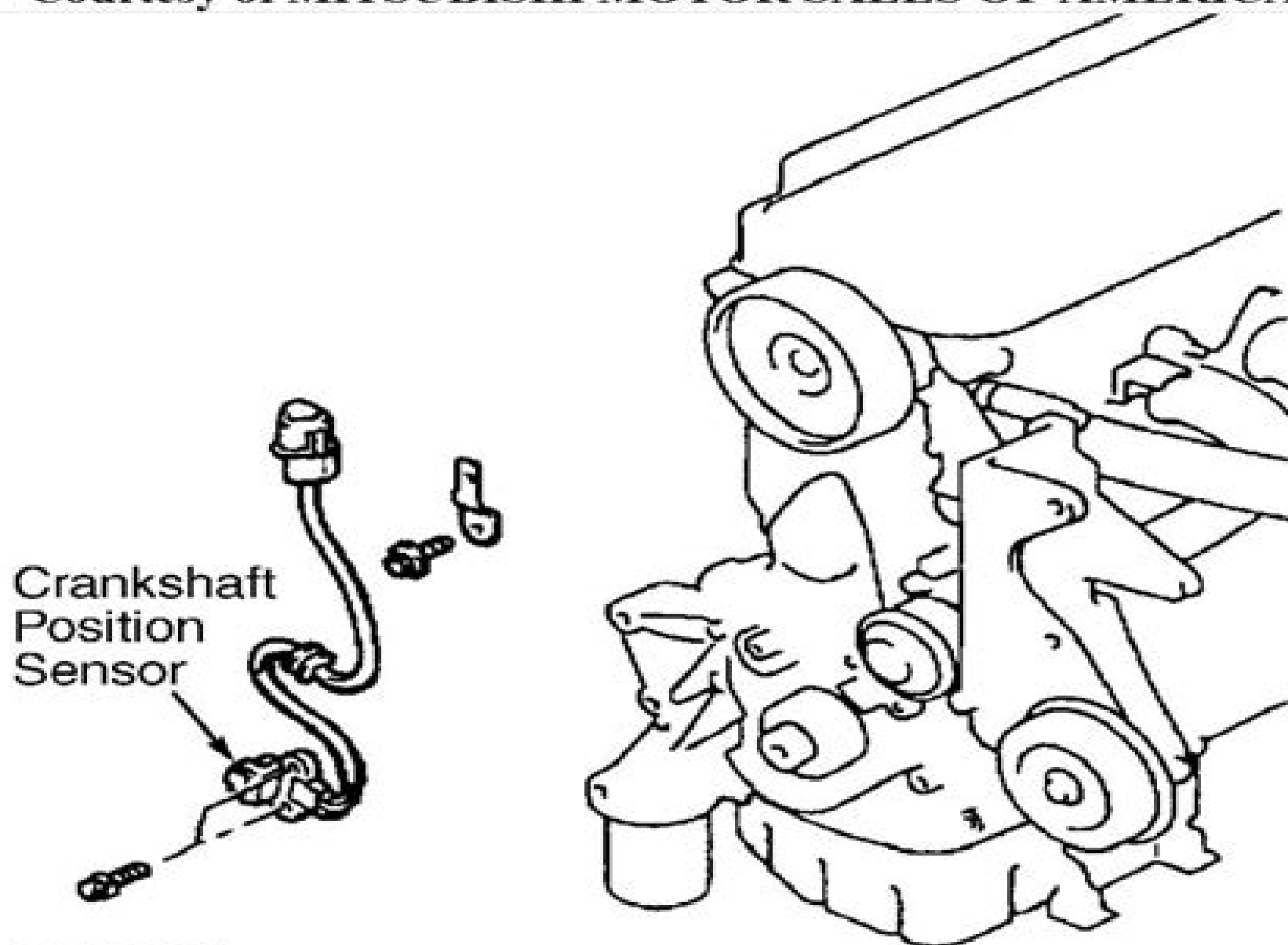
Fig. 57: Locating Crankshaft Position Sensor (Mirage 1.5L) Courtesy of MITSUBISHI MOTOR SALES OF AMERICA.
