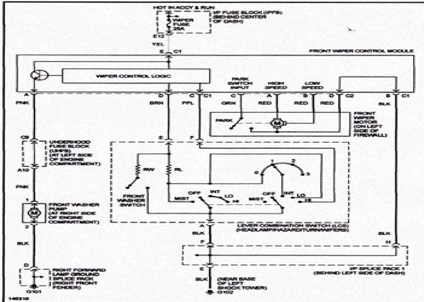
2001 Saturn SL2-Fig. 38: Front Washer/Wiper Circuit
