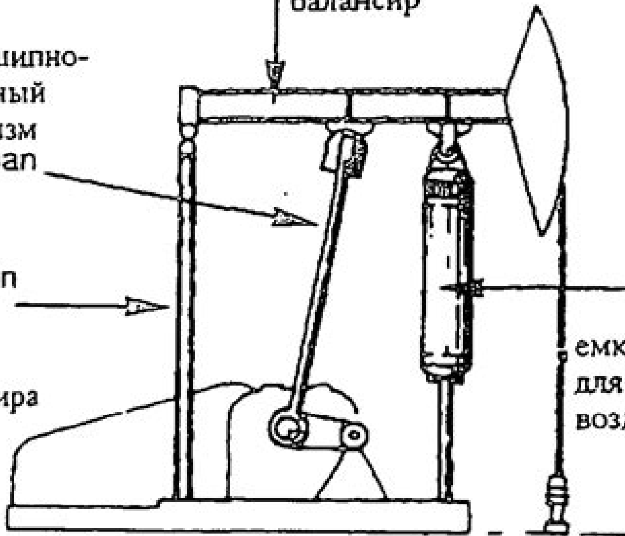
air balanced beam pumping unit
