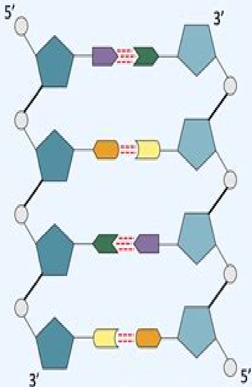
Antiparallel Strands
