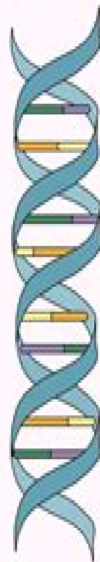
Double Helix
