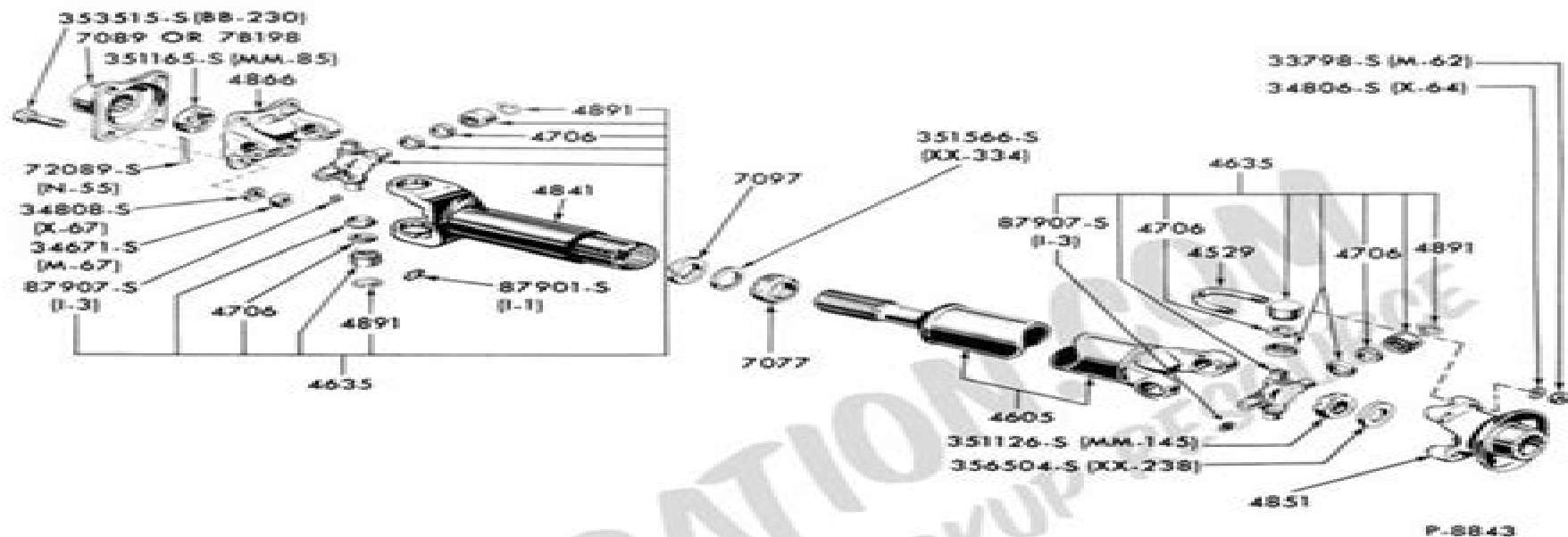
1964/72 SHORT WHEEL BASE DRIVE LINE - E100/300, F100/250, P100/350 - TYPICAL
