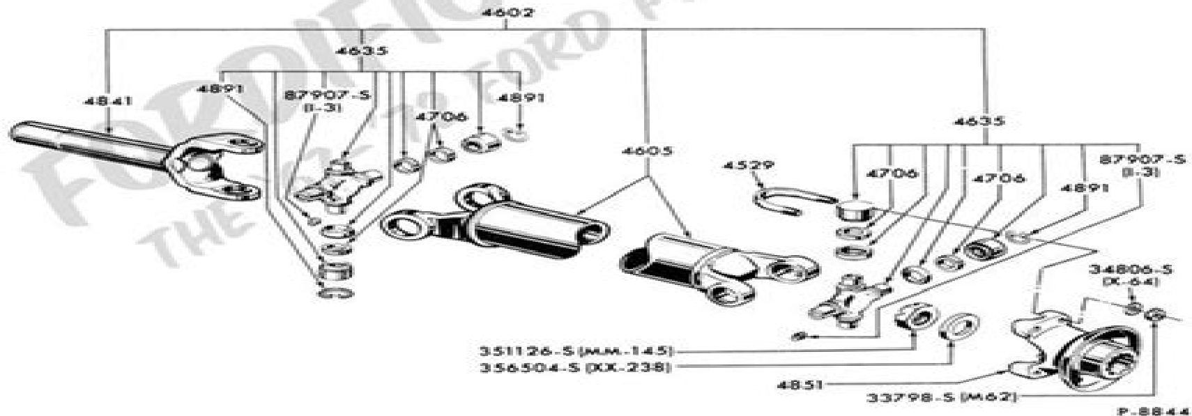
1964/72 DRIVE SHAFT (AUTOMATIC TRANSMISSION) - E100/300, F100/250
