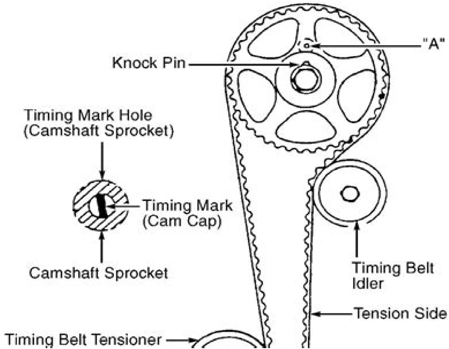
Fig. 1: Aligning Timing Marks Courtesy of HYUNDAI MOTOR CO.
