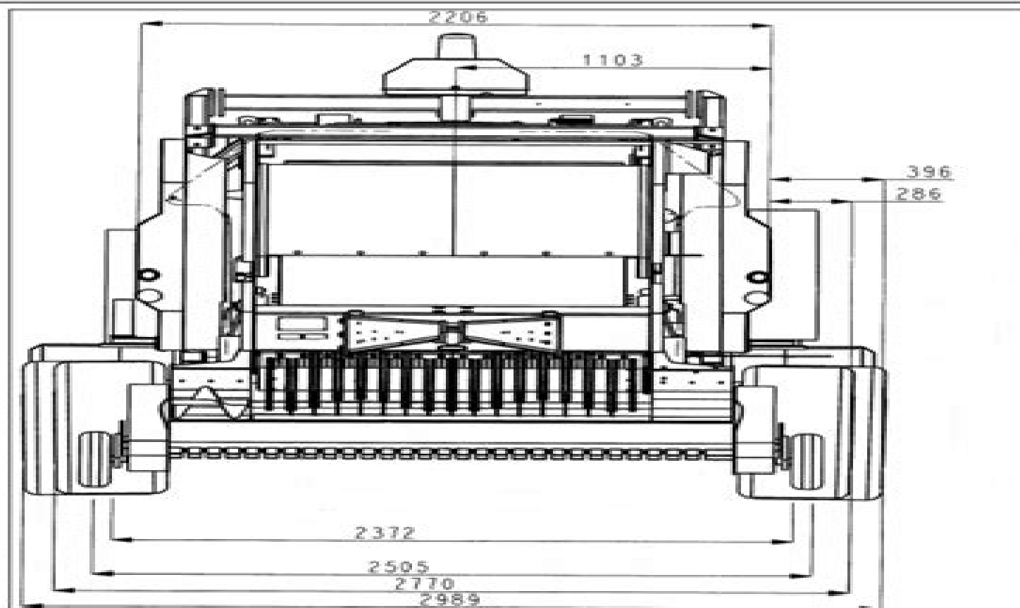
FIGURE 1 General Dimensions
