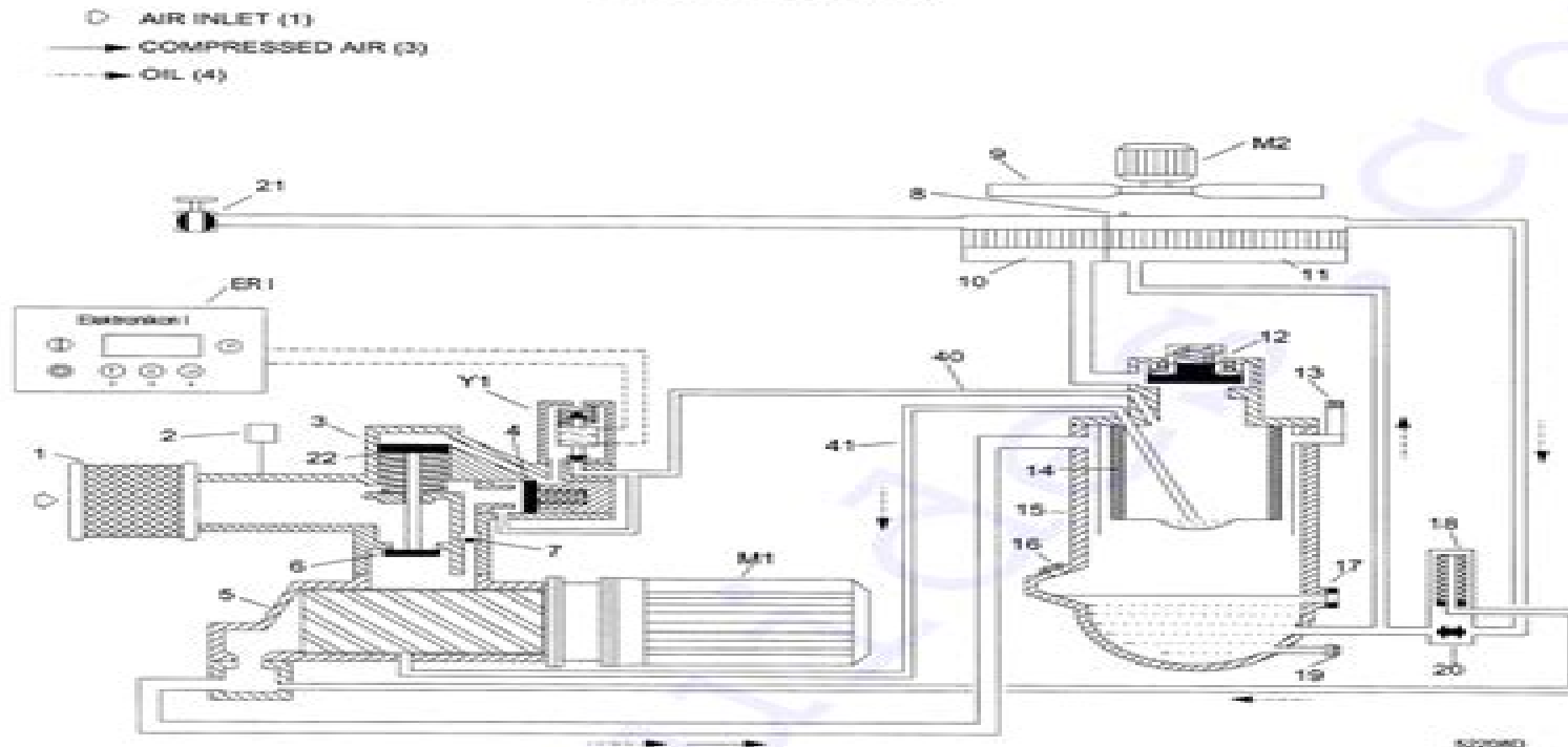
Fig. 1.8 GA Pack during unloading
