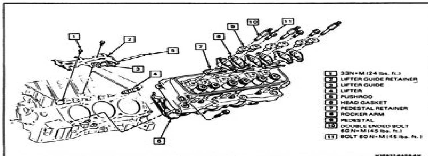
Figure 18 Valve Train & Cylinder Head
