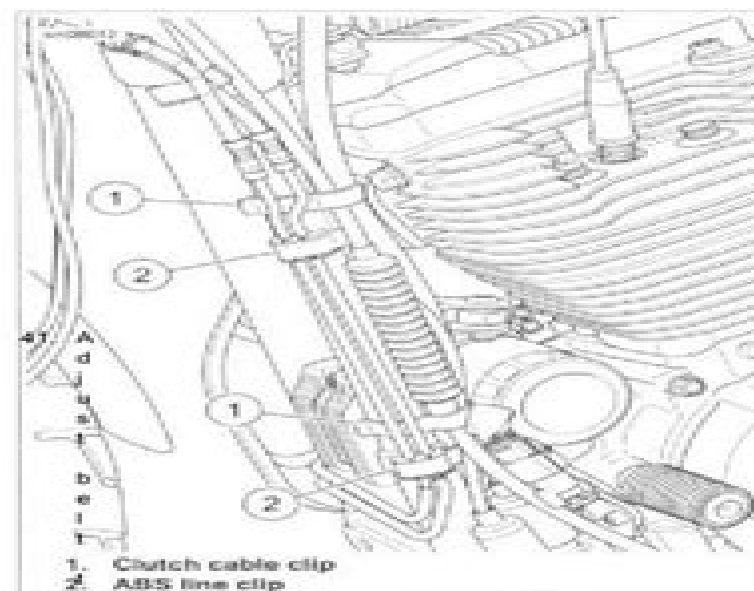
Figure 3-14. Frame Retaining Clips sion and rear wheel alignment. Tighten rear axle nut to 95-105 ft-lbs (129-142 Nm). Install new E-clip. See 1.20 WHEEL ALIGNMENT.
