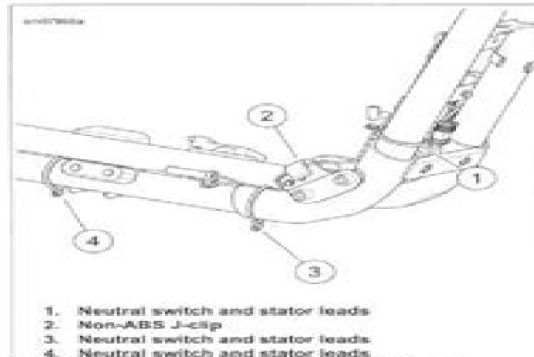
Figure 3-13. Lower Right Frame Tube Cable Straps
