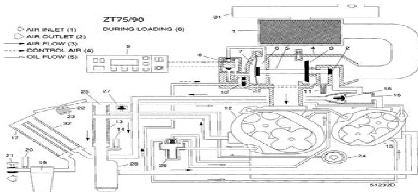
Fig. I.17 ZT75/90 during loading
