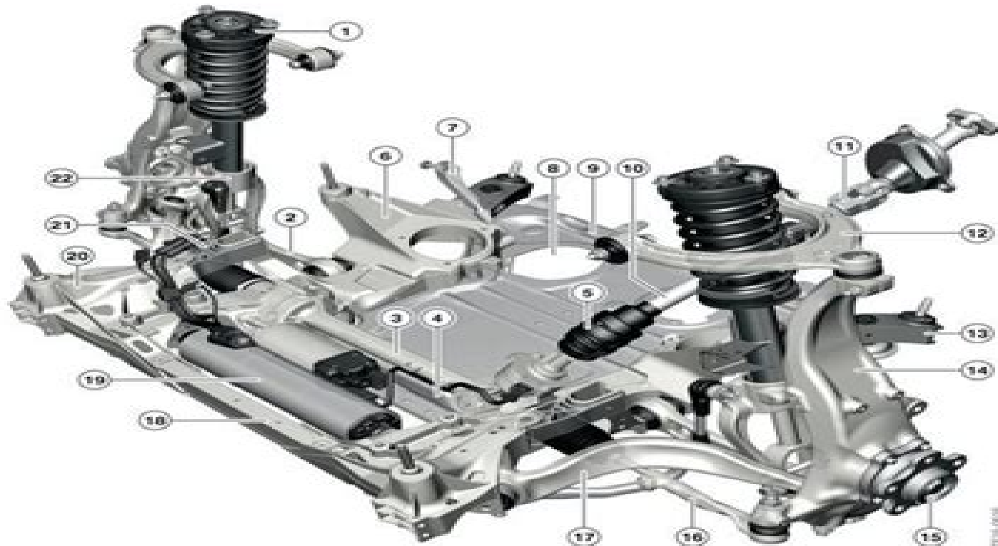
Double-wishbone front axle in the G30
