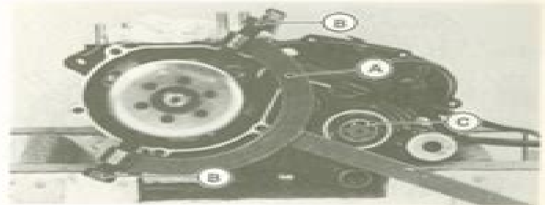
A. Rotor Holder: 57001-308 C. Sleeve B. Adapter "A": 57001-1108
