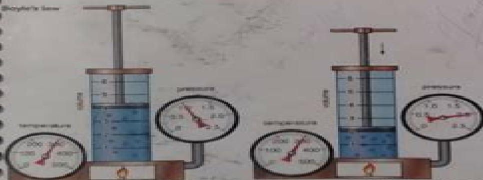
Boyle's Law
