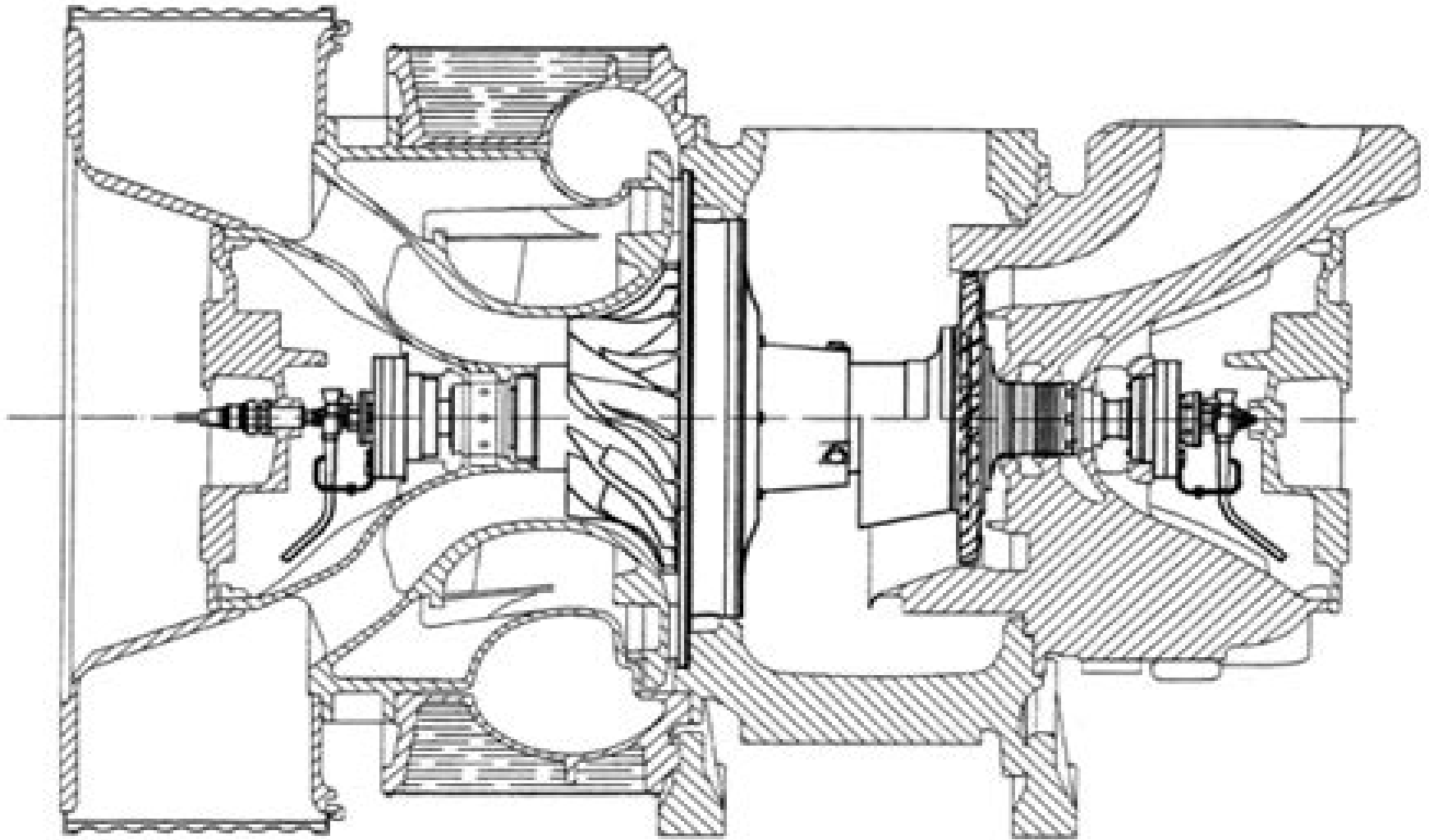
Turbocharger complete
