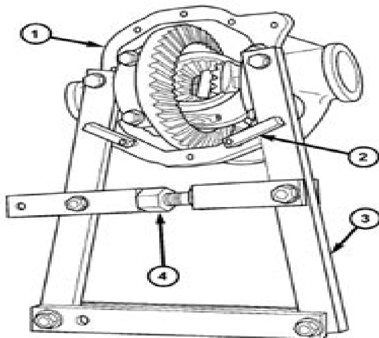
Fig. 37 DIFFERENTIAL SPREADER
