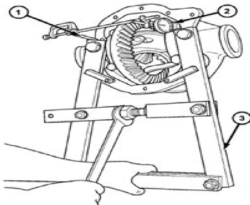
Fig. 38 SPREAD DIFFERENTIAL CASE
