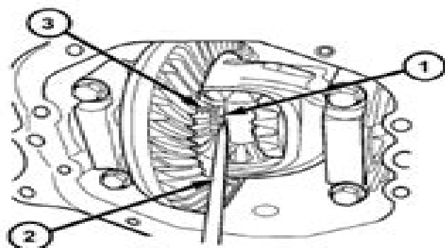
Fig. 36 RIGHT SHAFT IN SIDE GEAR
