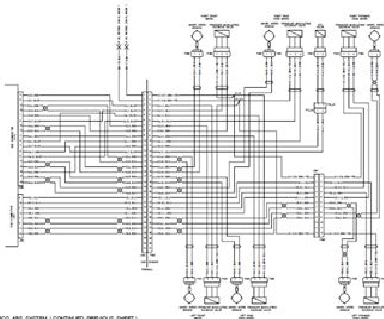
WABCO ABS SYSTEM (CONTINUED PREVIOUS SHEET)
