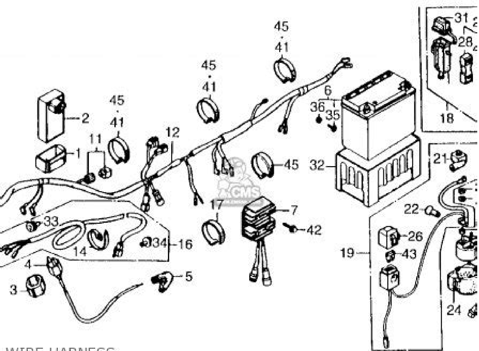
WIRE HARNESS
