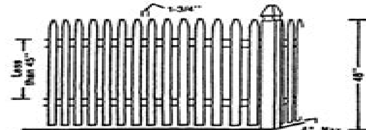
FIG. 1 If Horizontal Members are Less Than 45 in. Apart, Vertical Spacing Shall Not Exceed 1-3/4 in.
