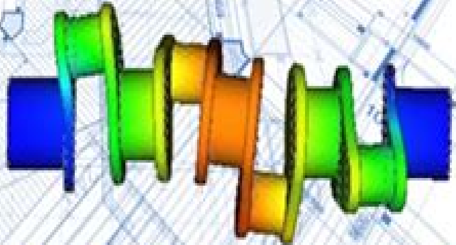
Mode Shape 2 - Frequency 151.7 Hz
