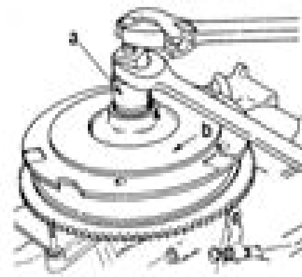
a - Flywheel Puller
