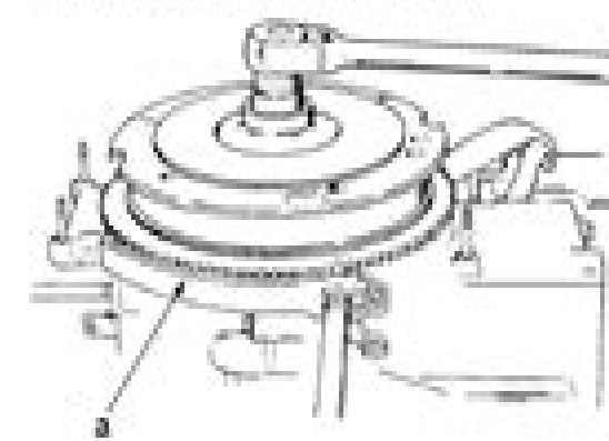
a - Flywheel Holder (91-52344)
